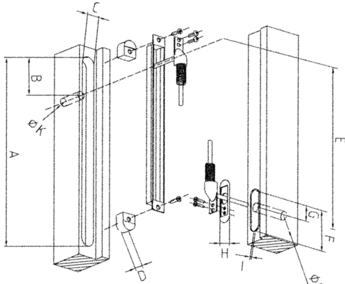
Pic. 3 Mounting in wood
