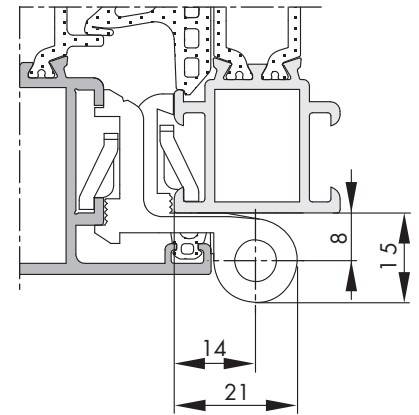
Point de rotation OF - LM
